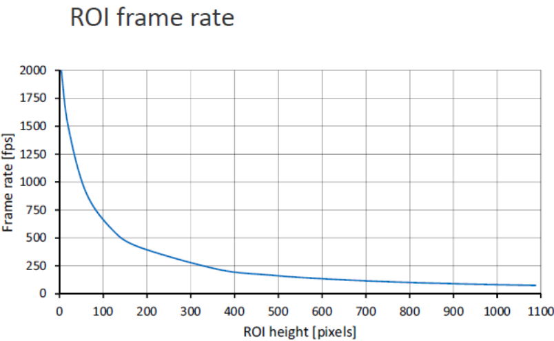
Figure 31: Frame rate as a function of ROI height
